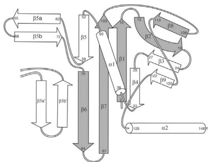
Figure 3 The topology diagram of the PA Nudix structure. The strand \beta 1 is connected by a type II \beta -turn to \beta 2 , which forms hydrogen bonds with the C-terminal part of \beta 1 and then makes a curve to form hydrogen bonds to \beta 3 , making a subsheet with strands \beta 8 and \beta 9 . A proline makes a kink at the end of \beta 3 , allowing \beta 4 to form hydrogen bonds to the N-terminal half of \beta 1 . A small loop connects \beta 4 to helix \alpha 1 . Strands \beta 5 and \beta 6 together form an almost continuous strand antiparallel to the longest strand \beta 7 . Strands \beta 5a and \beta 5b go to the other subunit and form part of its central \beta -sheet, while strands \beta 5a' and \beta 5b' are from the other subunit. The last helix \alpha 2 is connected to \beta 9 by a type I \beta -turn. There are more \beta -strands in this protein structure than in the E. coli MutT. The shaded \beta -strands are the strands that are present in the E. coli MutT structure.
