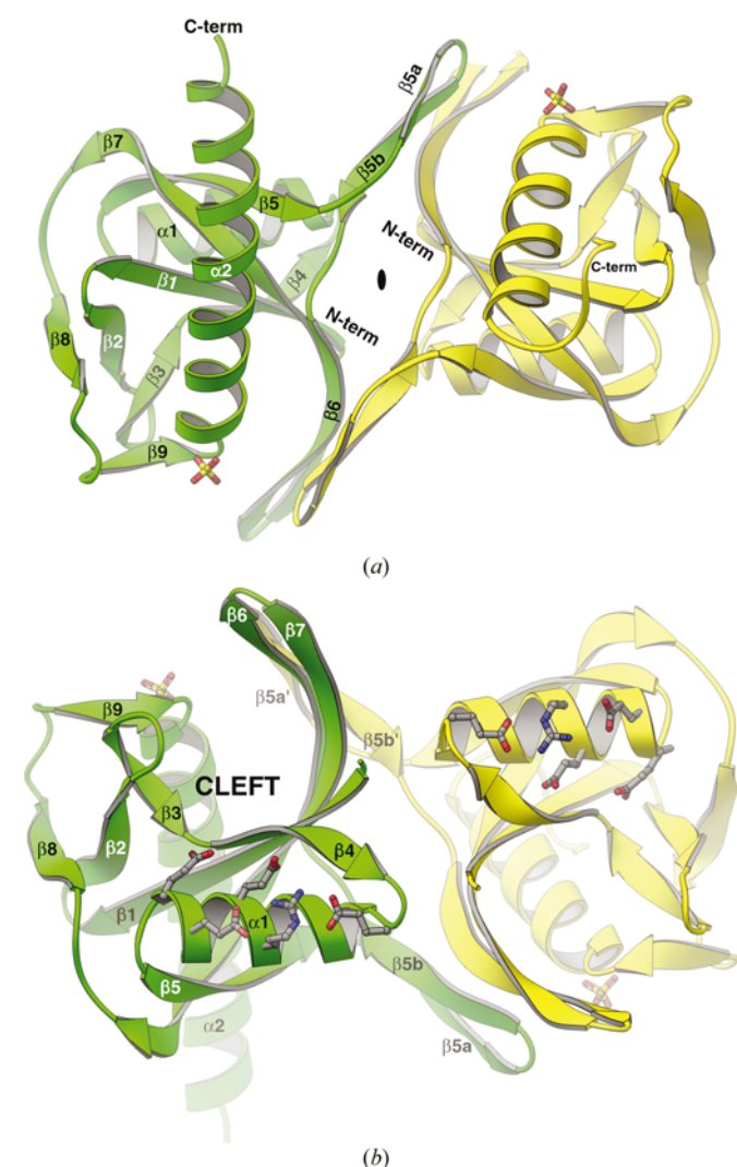
Figure 2 Ribbon diagrams of the PA Nudix structure. (a) shows the dimer with the twofold NCS axis perpendicular to the paper plane. Each subunit is composed of a long highly twisted central \beta -sheet and a small subsheet connected through strand \beta 2 , sandwiched between two \alpha -helices. Each subunit contributes two \beta -strands ( \beta 5a and \beta 5b ) to the \beta -sheet of the other subunit to form the dimer interface. Subunit A (on the left) has a long C-terminal helix \alpha 2 with the eight amino-acid linker at the C-terminal end extending the helix, while subunit B has a shorter helix \alpha 2 and its C-terminus and the linker fold back to form a more compact structure. (b) is a near 180^\circ rotation of (a) along a horizontal axis. A cleft formed by the \beta -strands connects helix \alpha 1 at the front to the N-terminal end of helix \alpha 2 at the back. The conserved arginine and glutamate side chains, as well as two sulfate ions found at the N-terminal end of \alpha 2 of each subunit, are shown as sticks. This figure was generated using RIBBONS (Carson, 1997).
