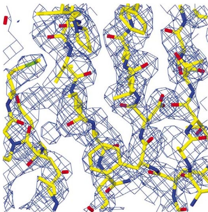
Figure 1 A section of the initial electron-density map superimposed on the final coordinates. The map was calculated at 2.5 Å with phases after twofold NCS averaging and contoured at 1.3\sigma . The figure was generated with the program O and rendered with POV-RAY .
